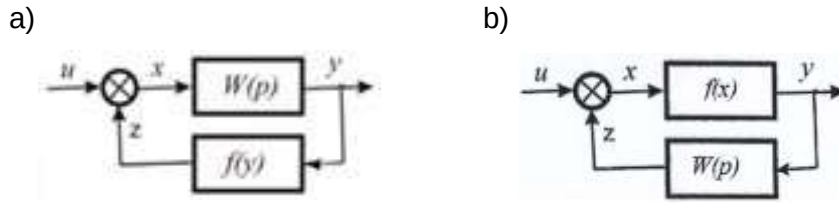
Fig. 1. The block-oriented models with feedback: a) linear model with nonlinear feedback, b) nonlinear model with linear feedback.
