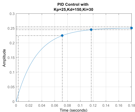
ბ) K_p = 25, K_d = 150, K_i=30;
